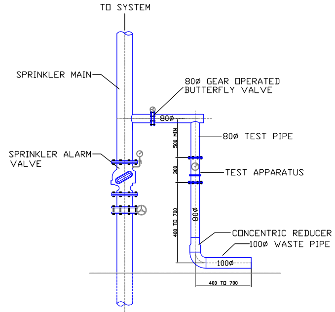
PROVING APPARATUS 7.5mm DENSITY
