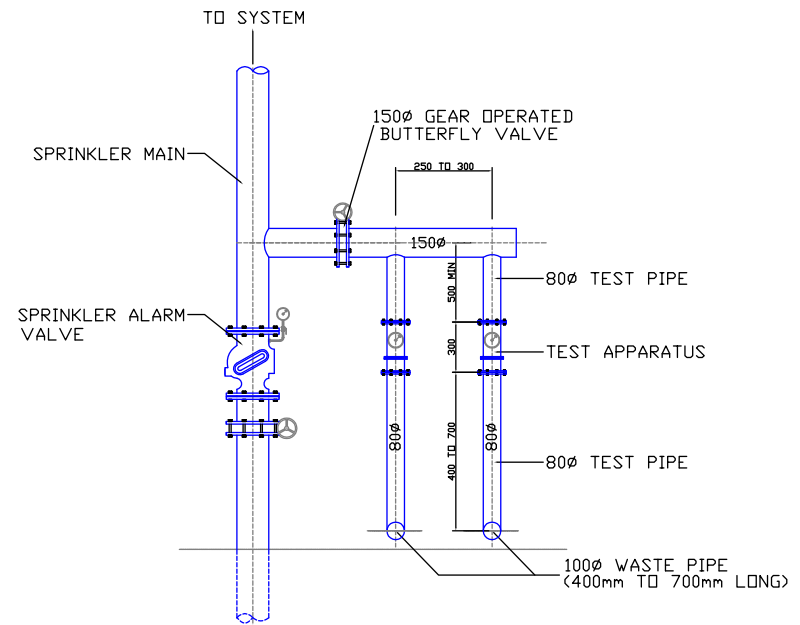
DUPLICATE PROVING APPARATUS ABOVE 10mm DENSITY
