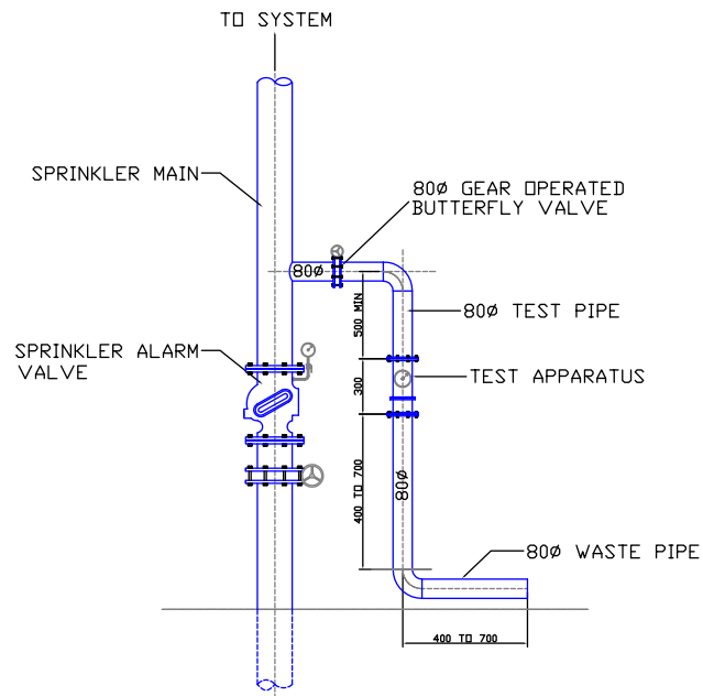
PROVING APPARATUS 5mm DENSITY
