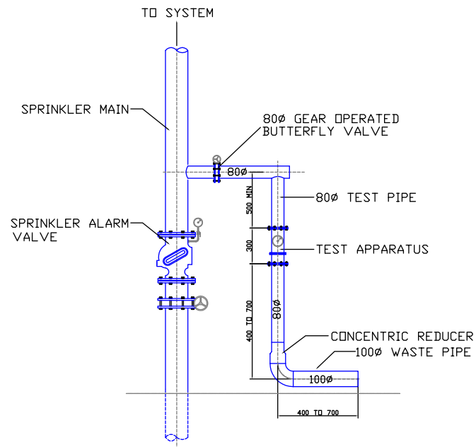
PROVING APPARATUS 10mm DENSITY
