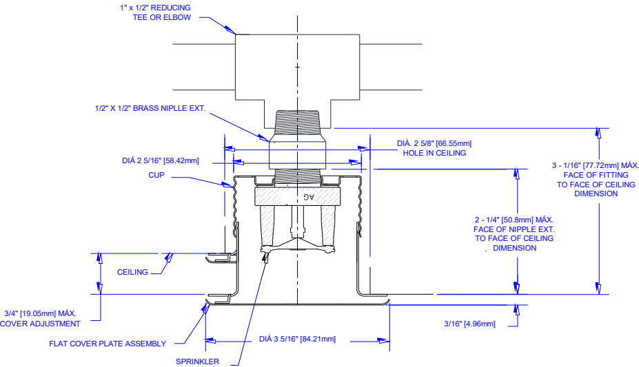
COVER PLATE, 3/4" (19 mm) ADJUSTMENT
