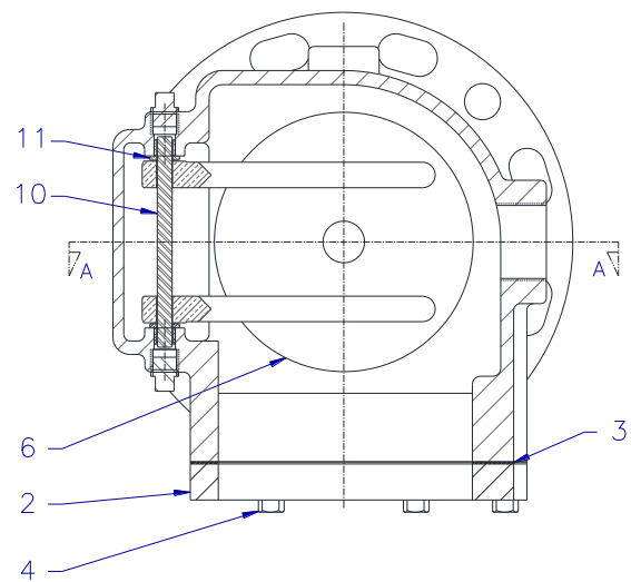
Lateral view
